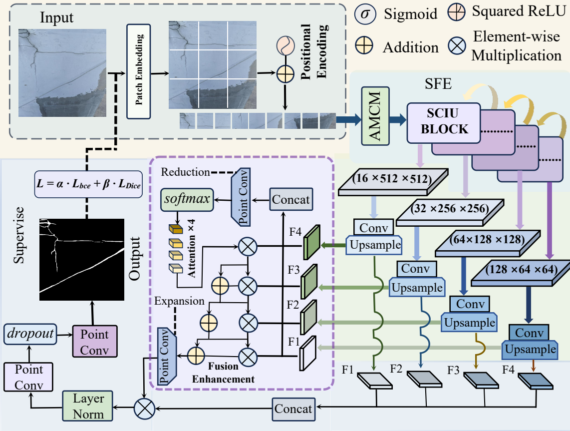
(a) Network Architecture of SCRWKV
