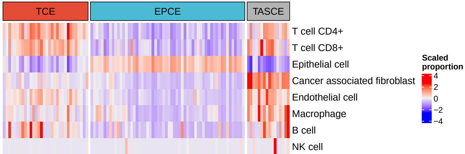
Cell type proportions across subtypes on the Atlanta dataset
