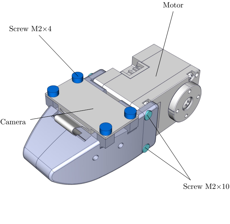
Assembled View
