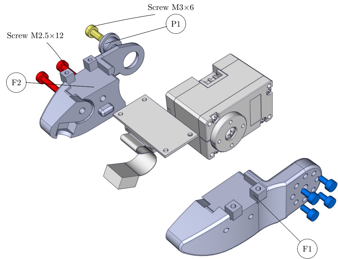
Exploded View
