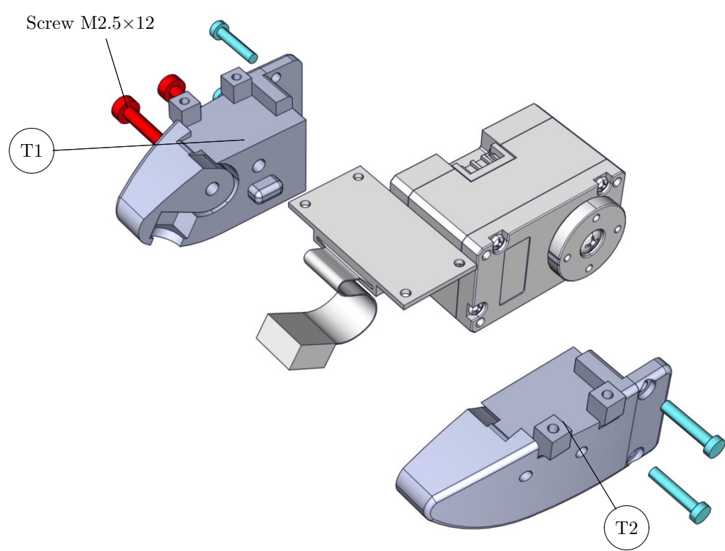
Exploded View
