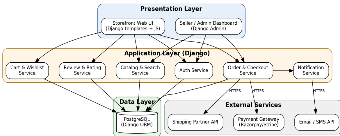
Figure 1: Component diagram of the Online Bookstore
