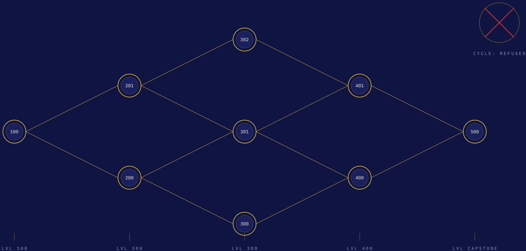
FIG. IV - PREREQUISITE GRAPH - ACYCLIC BY PROOF
