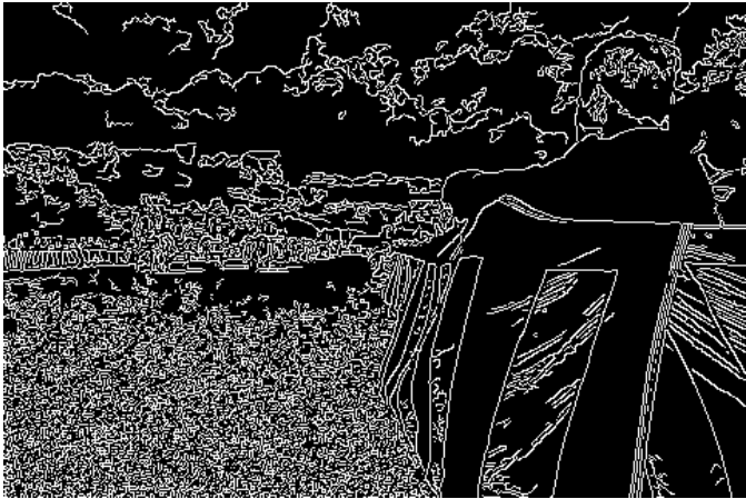
Output Image
