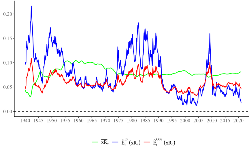
Figure 6: Time series of sample mean, IS and restricted OS estimates
