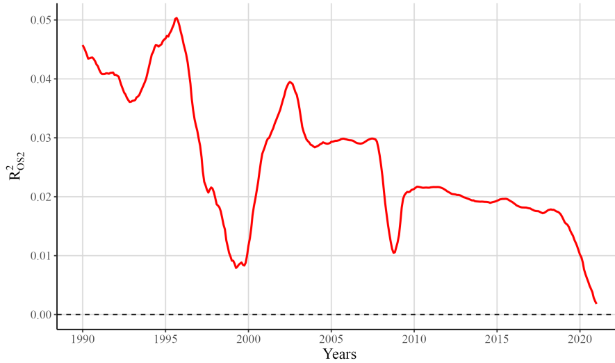
Figure 7: Rolling 50-year restricted out-of-sample R-squared
