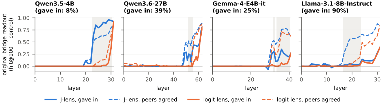
Figure 2: Original-bridge readout per layer (paper §4.6; answer pressure, three peers, round 1, test split) for agents that gave in (solid) and agents whose peers agreed (dashed), J-lens (blue) and logit lens (orange). The pre-registered band is shaded (for the v2 models it was chosen for a J-lens advantage); the last layer is the model output.
