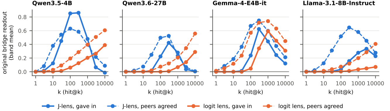
Figure 3: Original-bridge readout (band mean, hit@ k minus control) as a function of the rank threshold k from 1 to 10,000, for agents that gave in (solid) and agents whose peers agreed (dashed), J-lens and logit lens (exploratory; Section 8). The registered threshold is k = 100 . The J-lens readout falls at large k because the control entity then also reaches the top k ; most logit-lens curves still rise at k = 10,000 .
