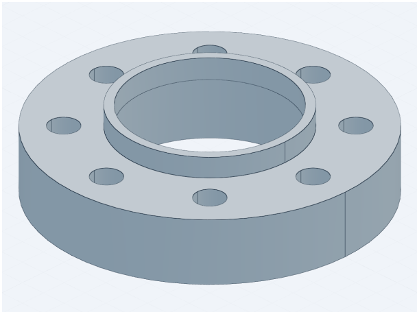
MK-008 iso9409_tool_flange 42CrMo | Qty 1 | 144x144x37.0 mm
