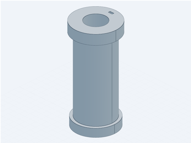
MK-005 j2_hollow_output_shaft 42CrMo | Qty 1 | 111.6x111.6x235.2 mm
