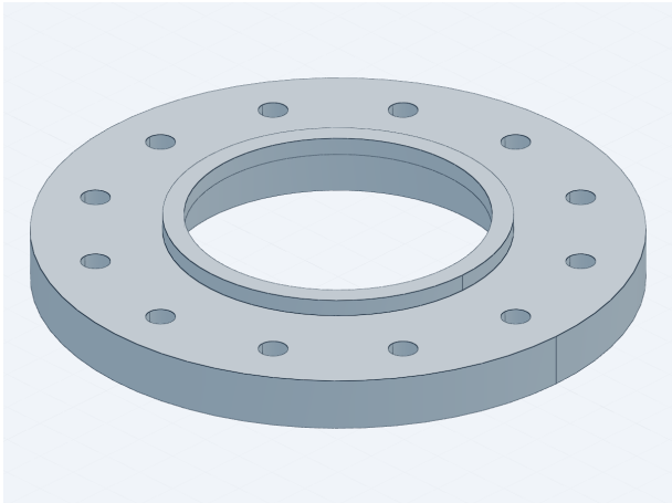
MK-006 j2_bearing_end_cover Q355B | Qty 1 | 270x270x31.7 mm
