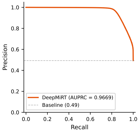
(B) Precision-Recall Curve
