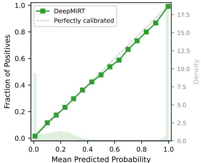
(C) Calibration (ECE = 0.0064)
