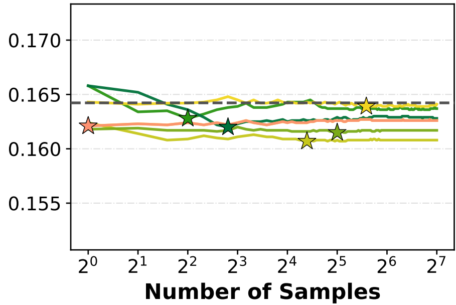
TimeMoE
