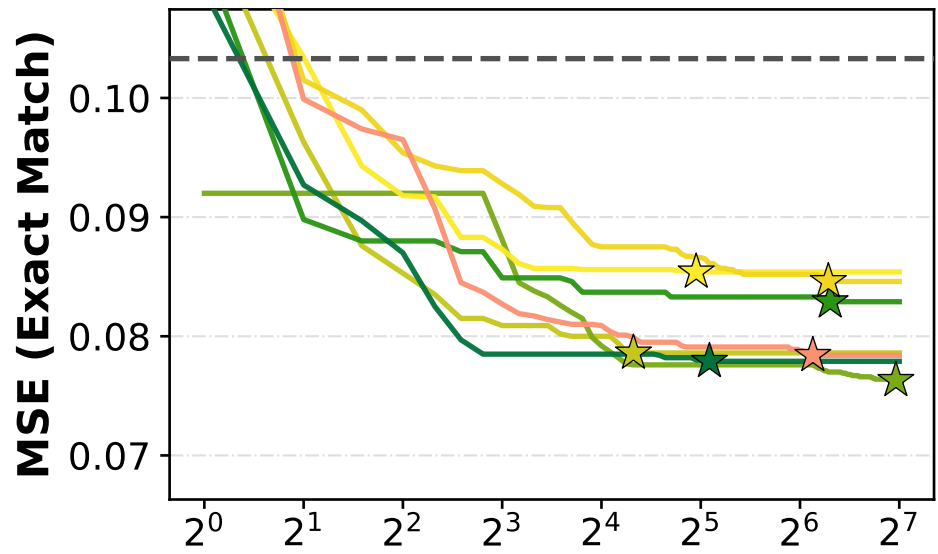
Chronos
