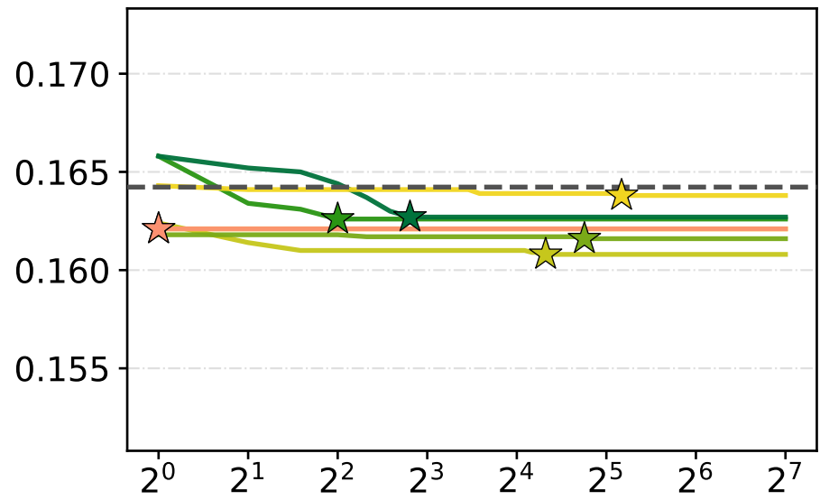
TimeMoE
