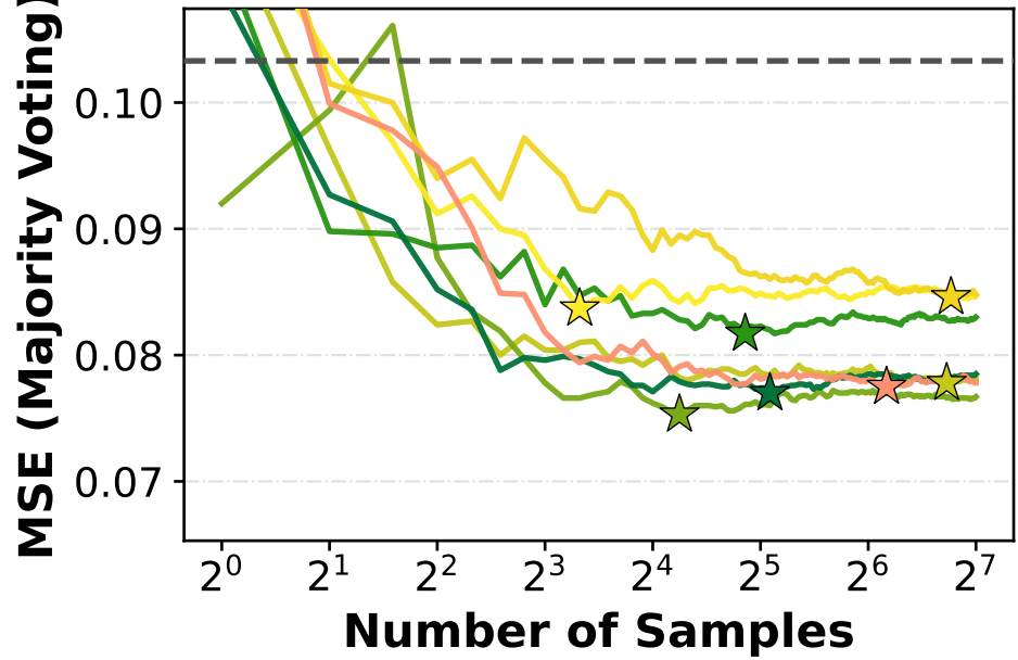
Chronos
