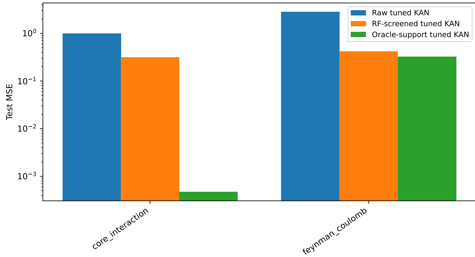
Tuned KAN: Test MSE
