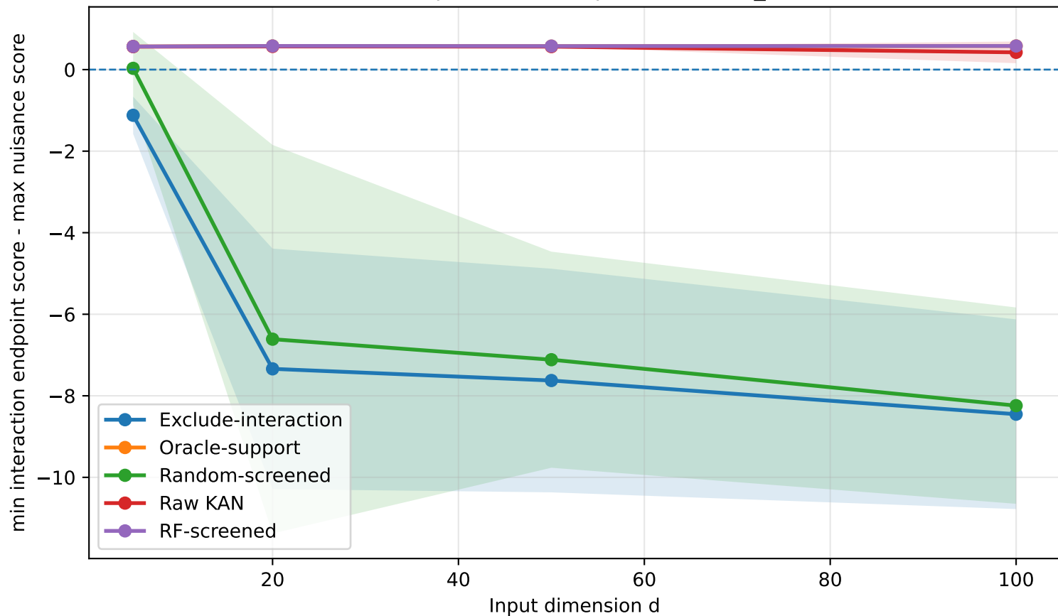
Interaction-endpoint score separation: core_interaction
