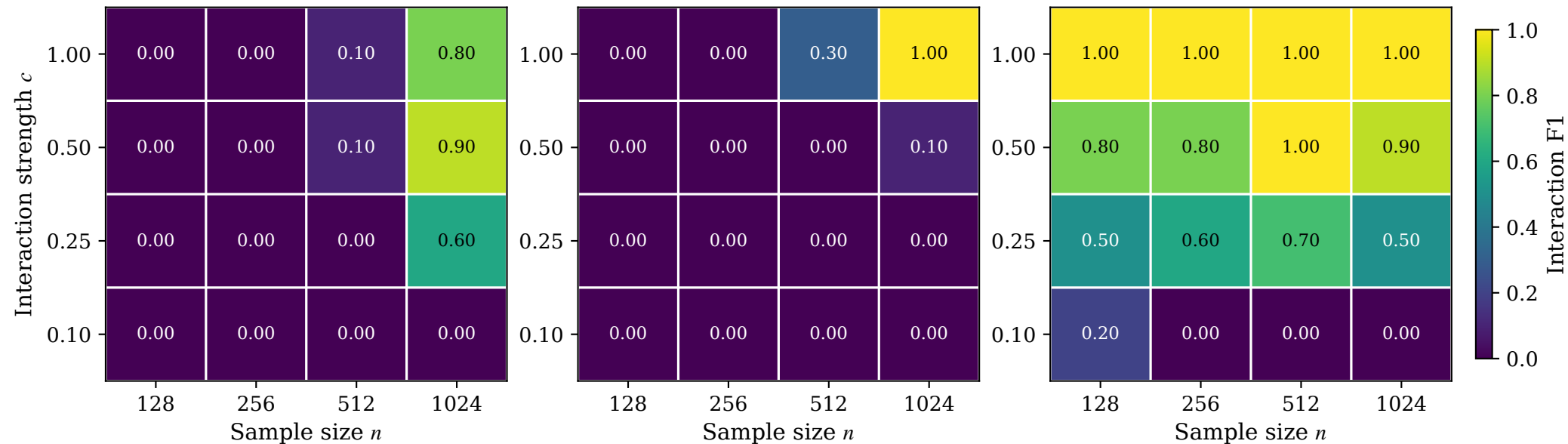
Formula-fidelity recovery boundary under nuisance dimensions ( d=100 )
