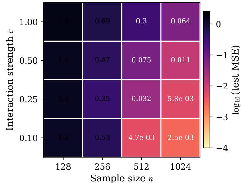
Prediction improves before formula recovery: Raw KAN ( d=100 )
