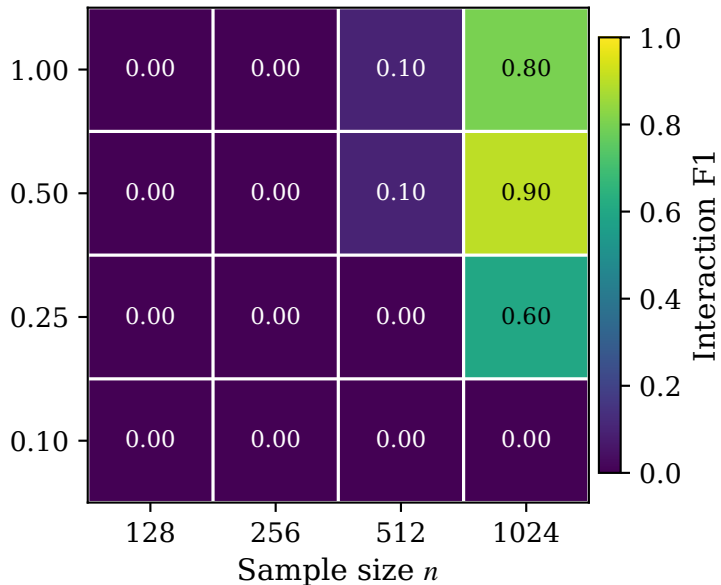
Prediction improves before formula recovery: Raw KAN ( d=100 )
