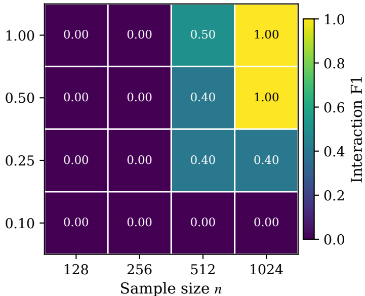
Prediction improves before formula recovery: Raw KAN ( d=50 )
