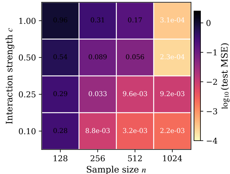
Prediction improves before formula recovery: Raw KAN ( d=50 )
