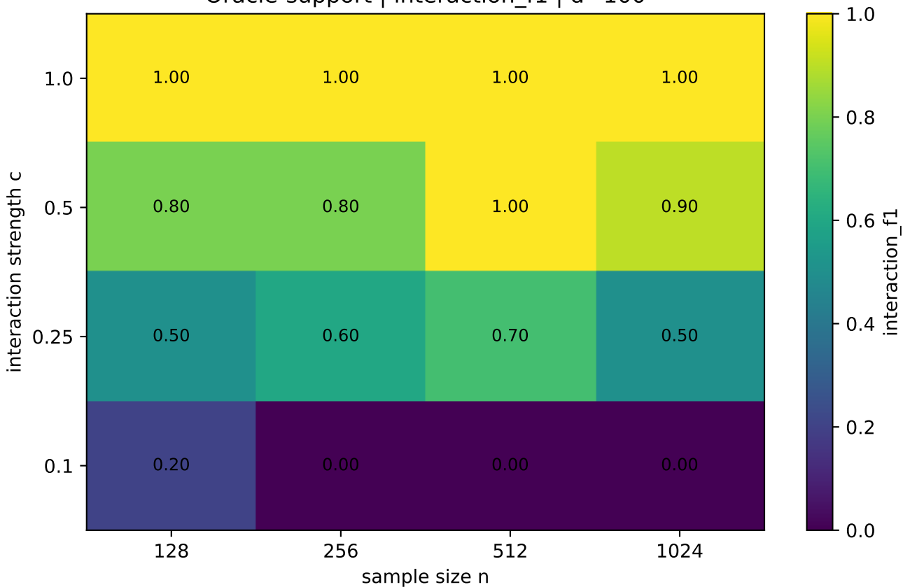
Oracle-support | interaction_f1 | d=100
