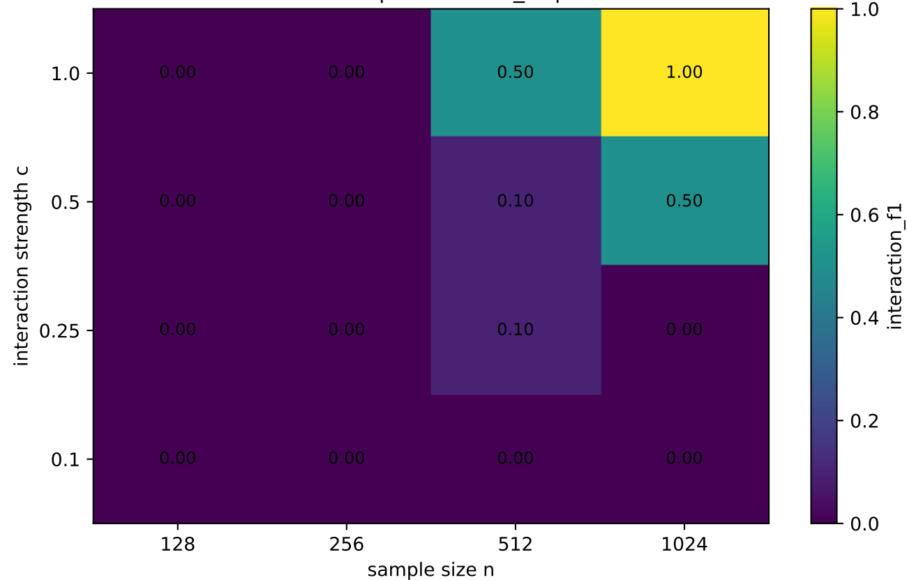
RF-screened | interaction_f1 | d=50
