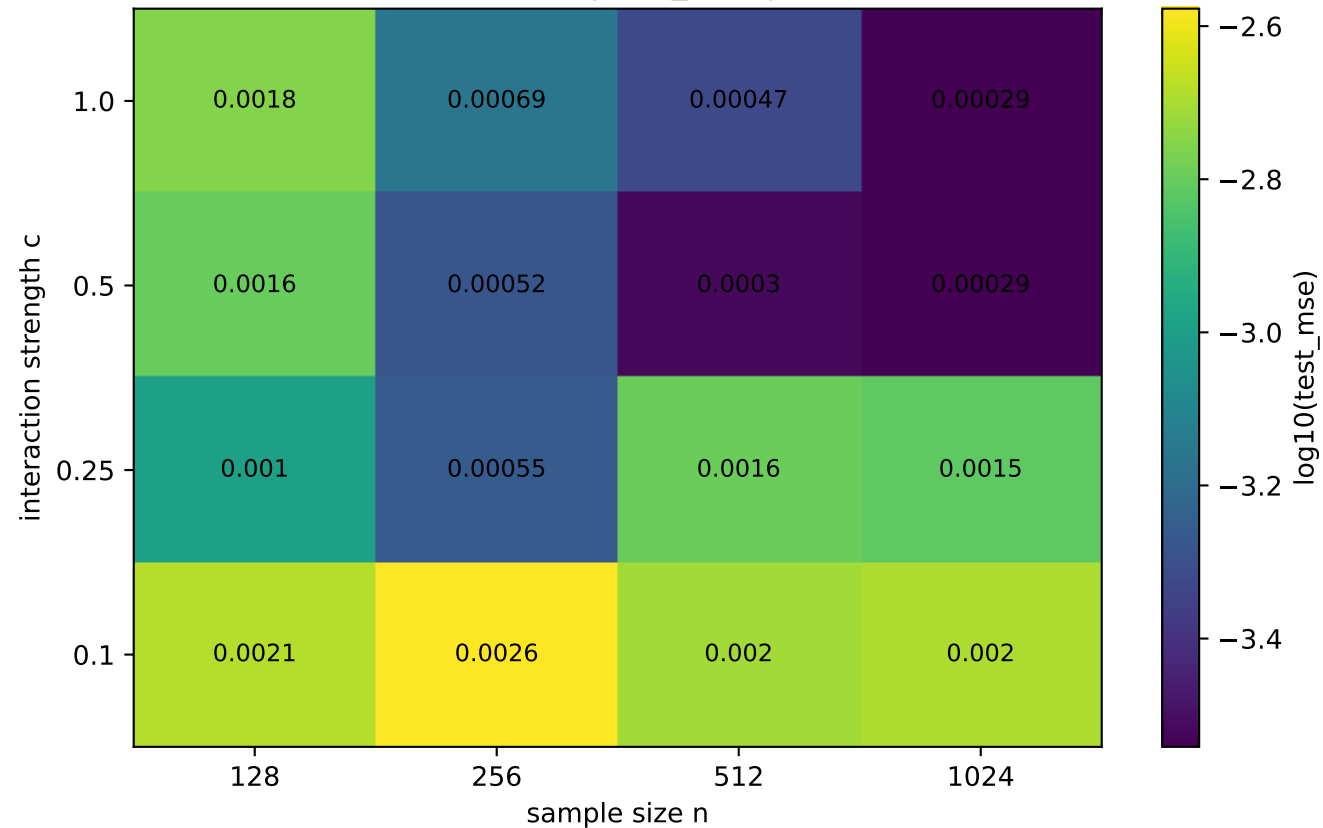
Oracle-support | test_mse | d=100
