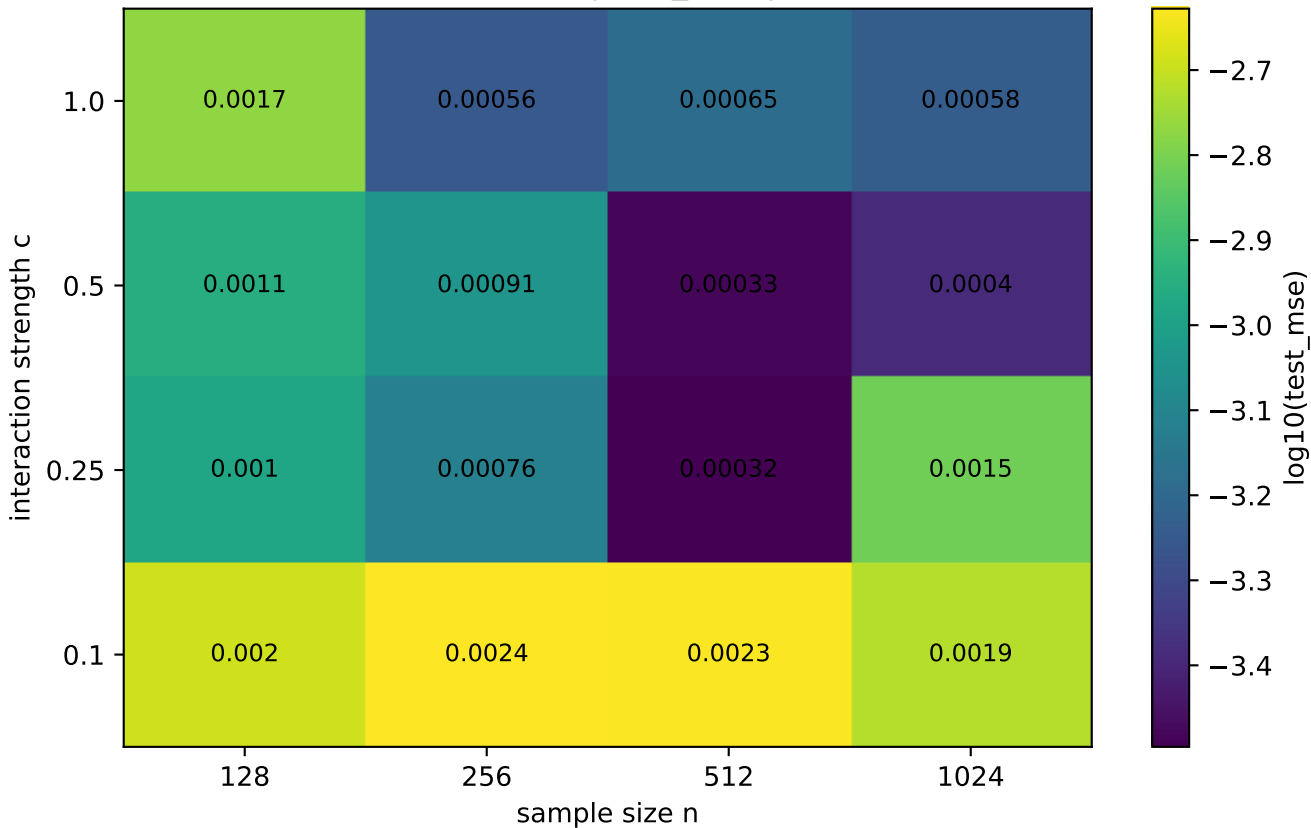
Oracle-support | test_mse | d=50
