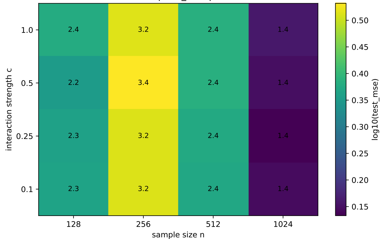
Random | test_mse | d=50
