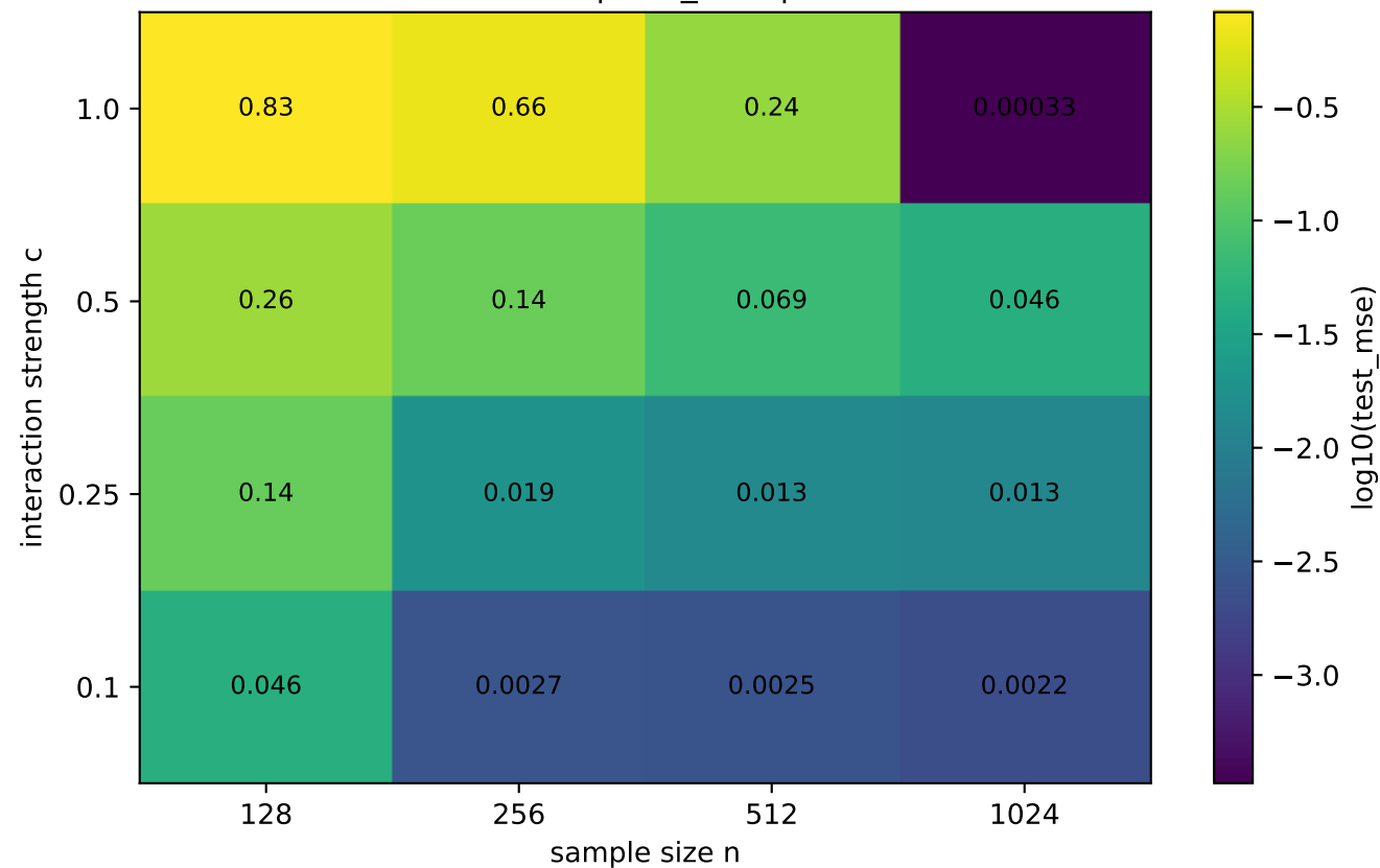
RF-screened | test_mse | d=100
