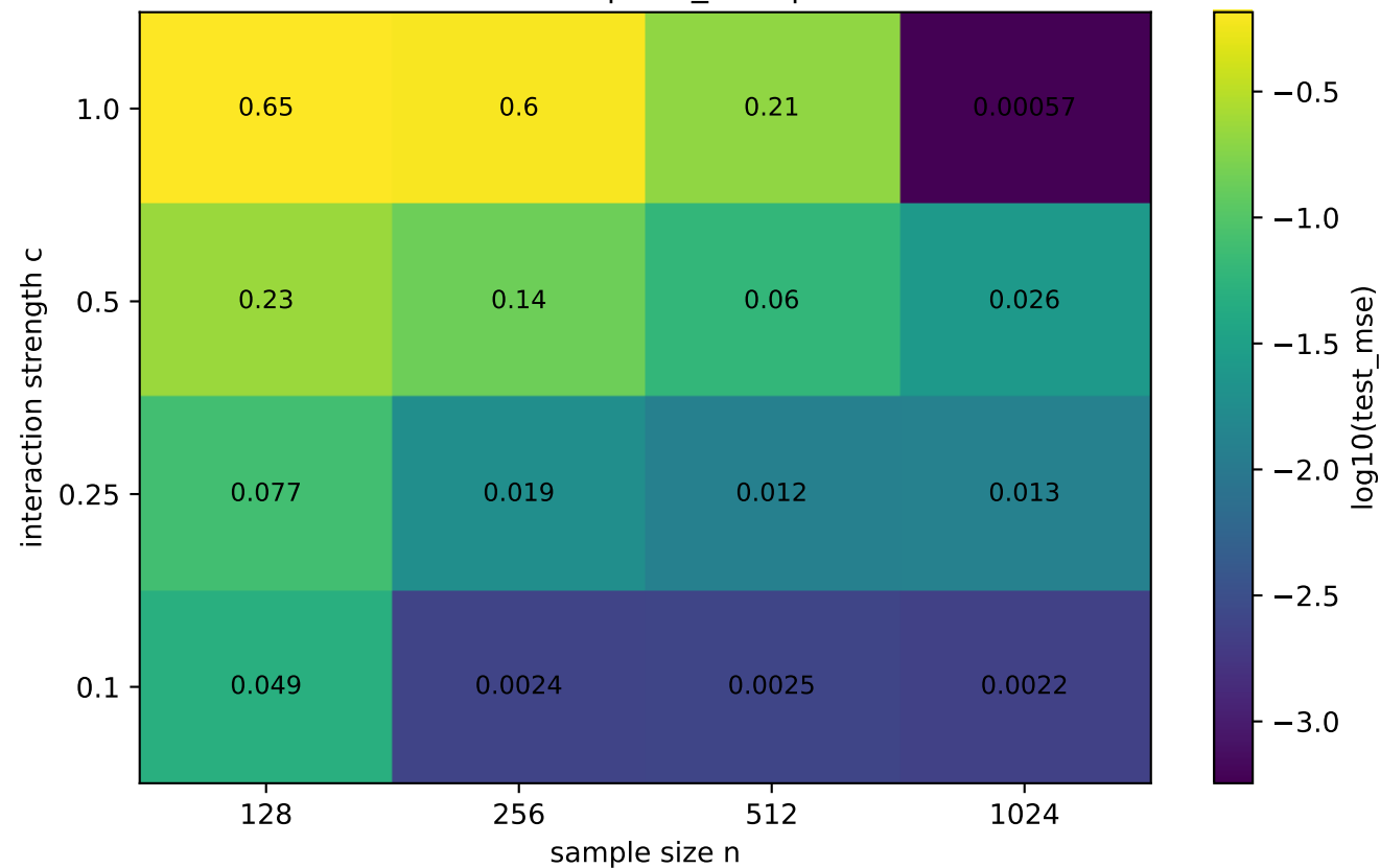
RF-screened | test_mse | d=50
