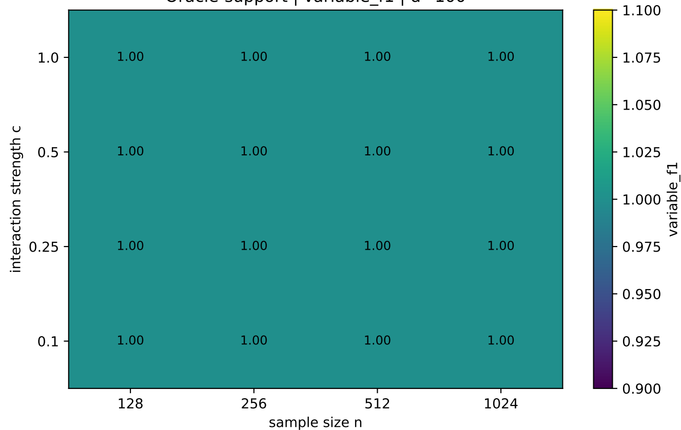
Oracle-support | variable_f1 | d=100
