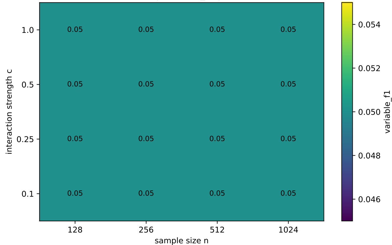
Random | variable_f1 | d=50
