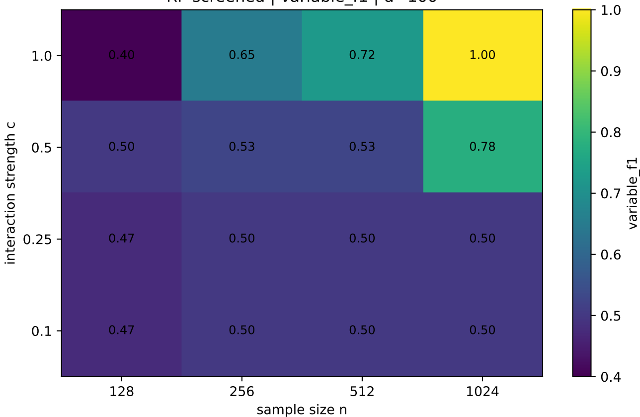
RF-screened | variable_f1 | d=100
