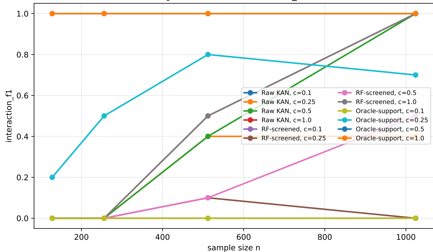
Hard-regime transition: interaction_f1, d=50
