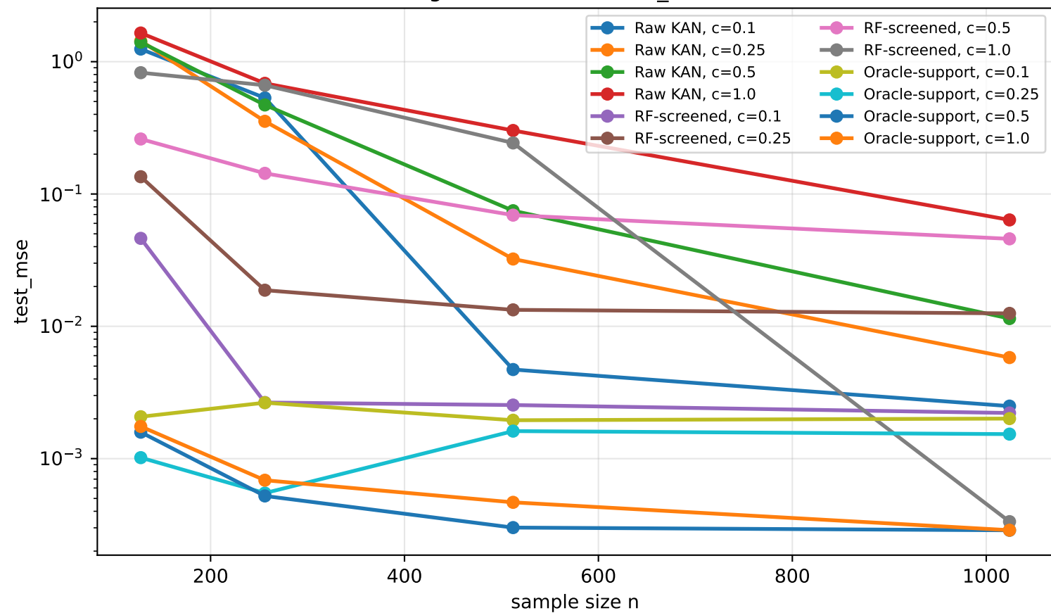
Hard-regime transition: test_mse, d=100
