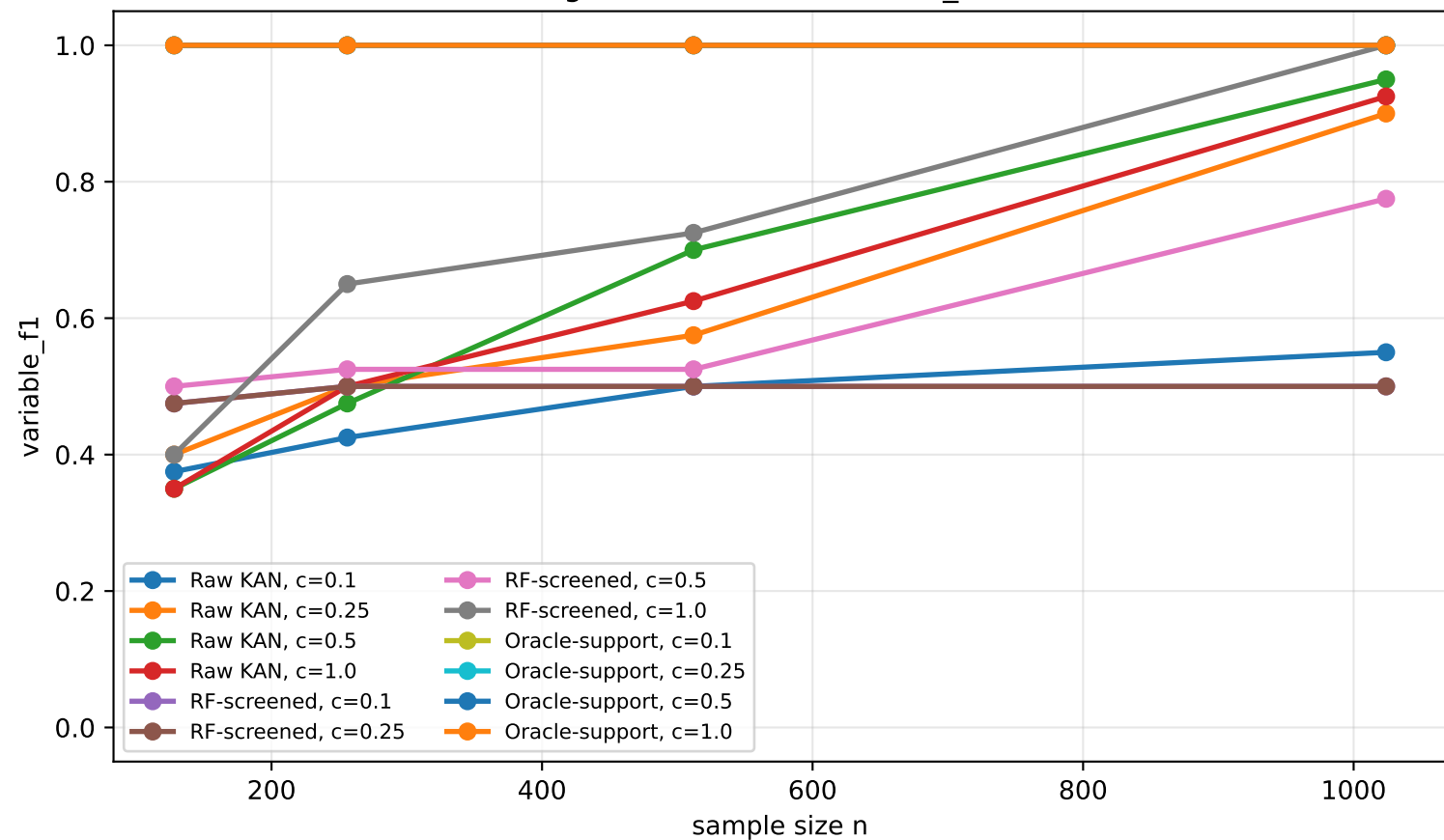
Hard-regime transition: variable_f1, d=100
