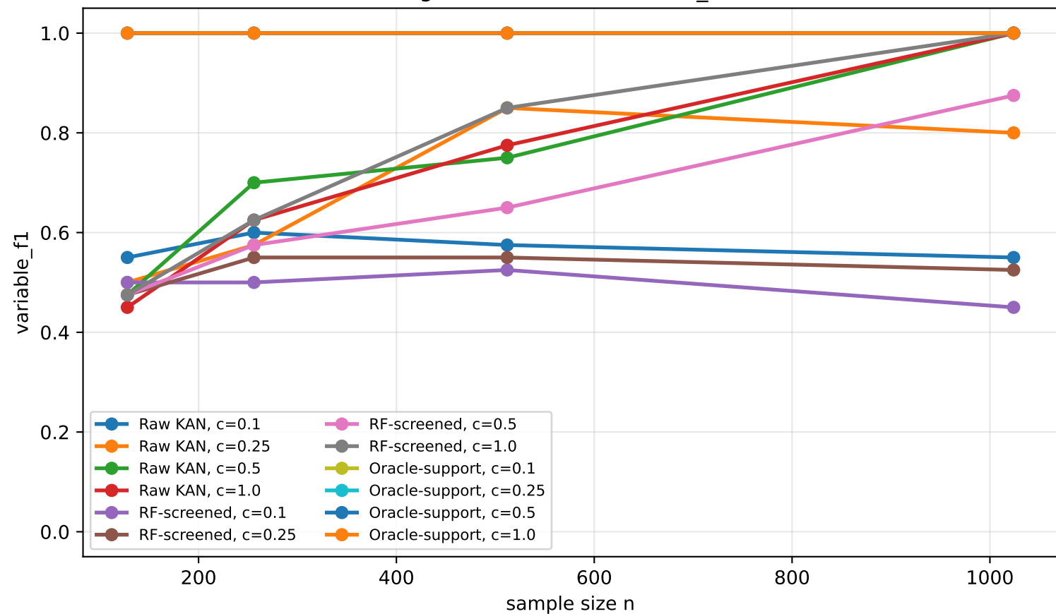
Hard-regime transition: variable_f1, d=50
