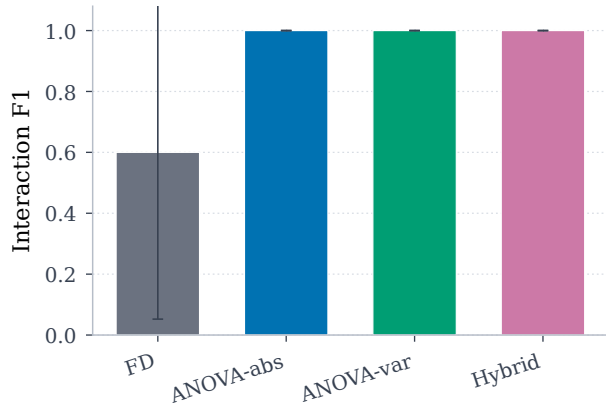
Pair Scoring After Oracle Support
