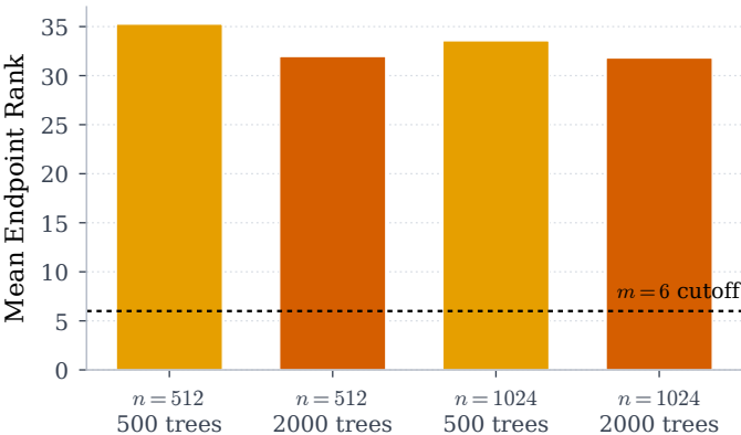
RF Marginal Screening
