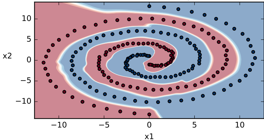
Decision boundary
