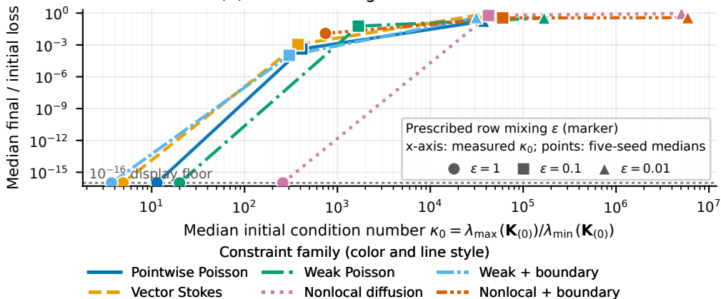
(b) Ill-conditioning slows finite-horizon GD
