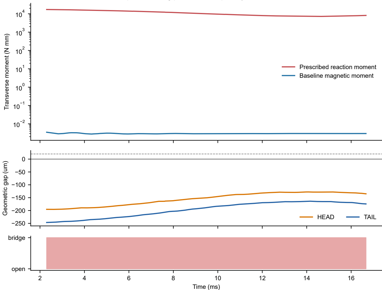
The imposed 30 deg path activates penalty-scale wall reaction
