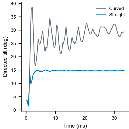
a Tilt response
