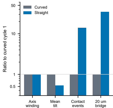
c Cycle-level comparison
