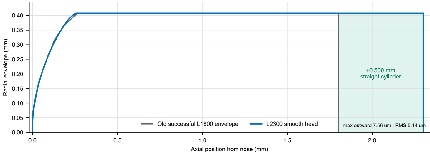
L2300 preserves the old head envelope and extends only the straight body
