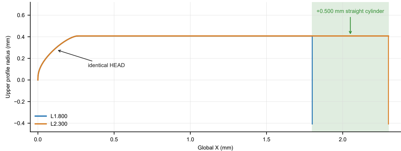
Length parameterization changes only the straight body
