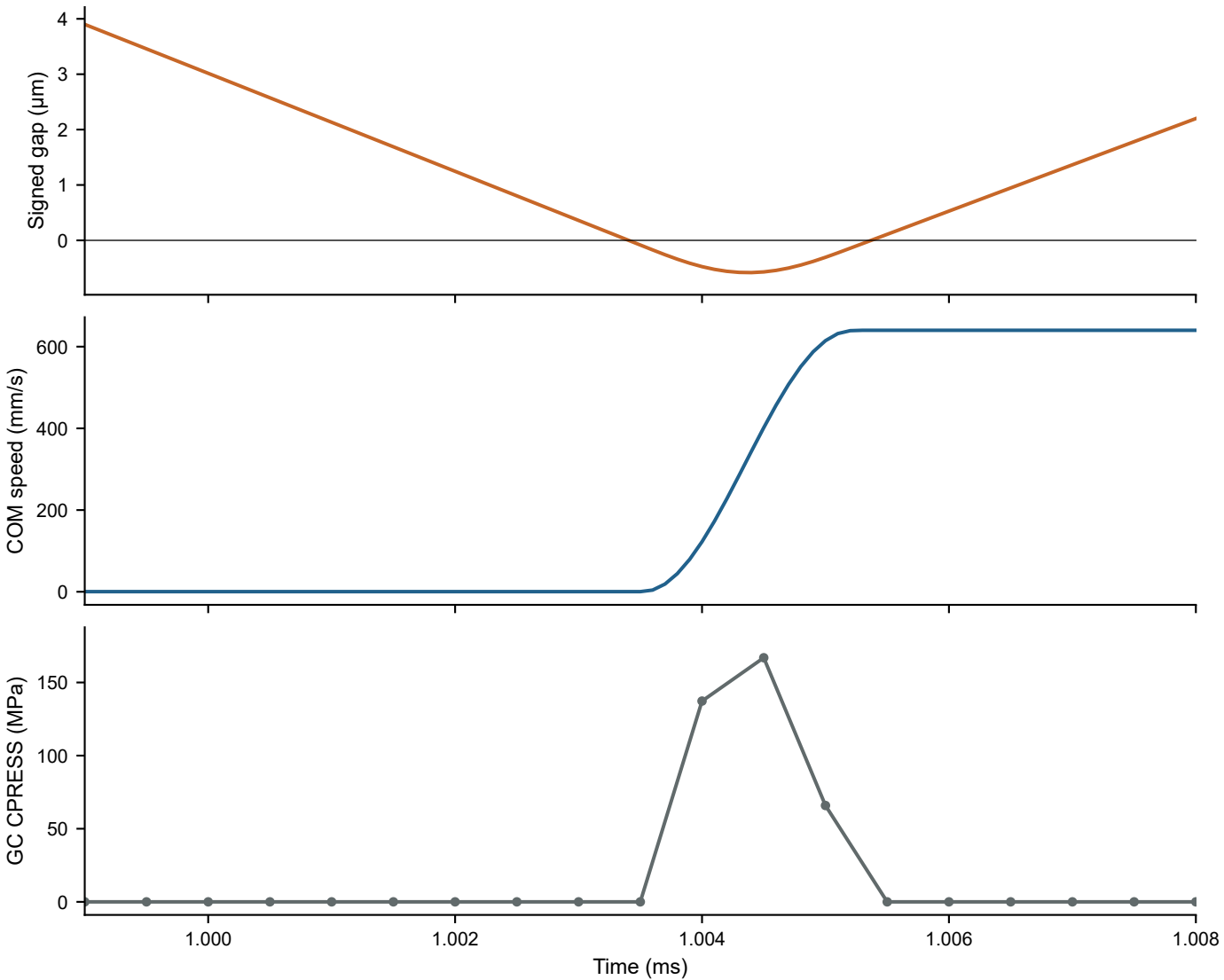
First impact: penetration, velocity jump and 0.5-us contact frames
