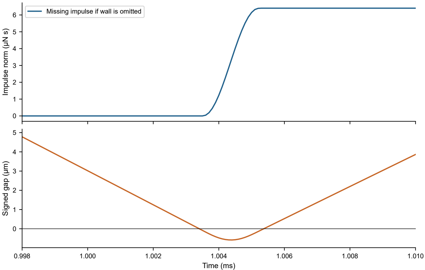
Momentum deficit grows during the near-wall rebound
