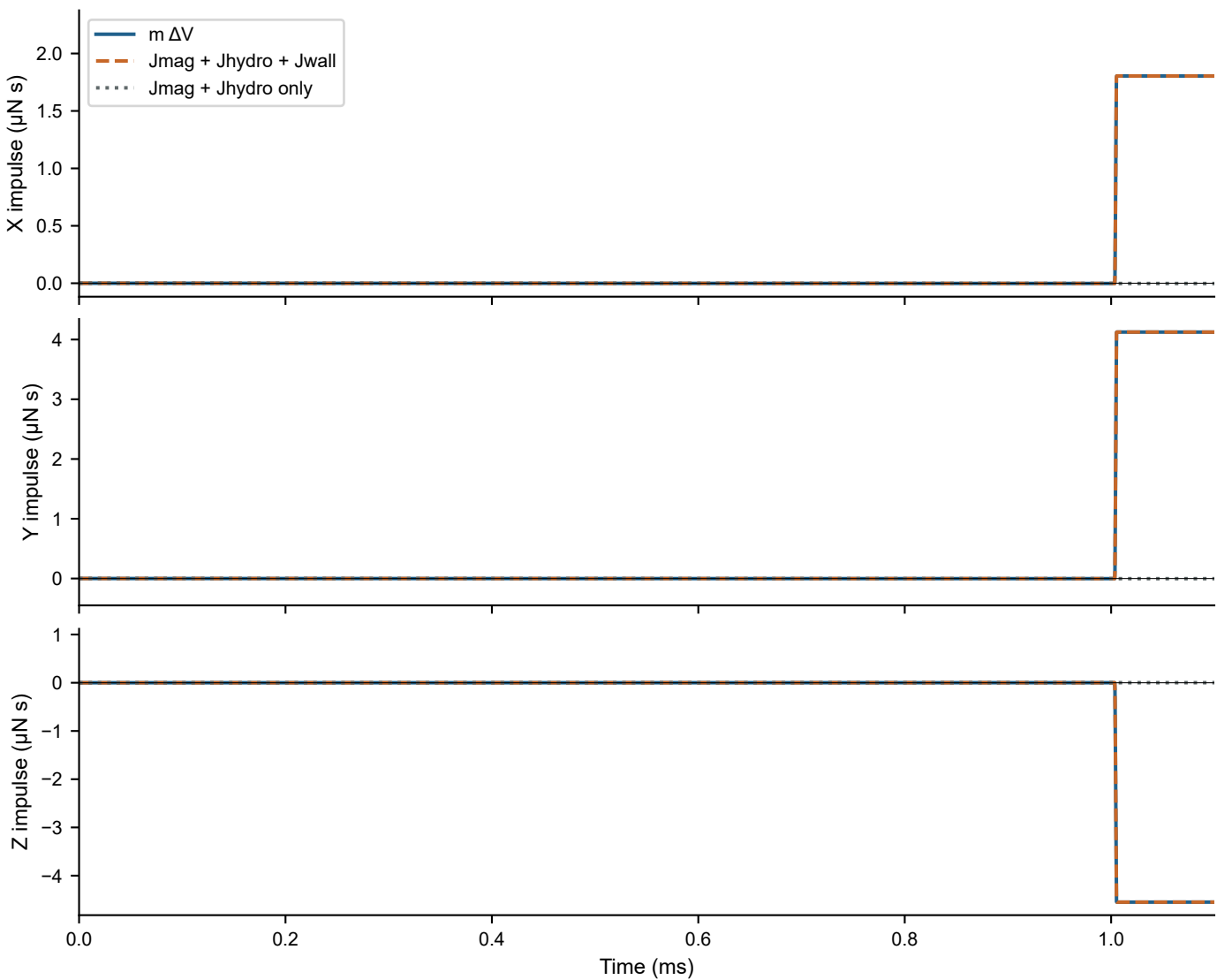
Independent wall-force output closes all three momentum components
