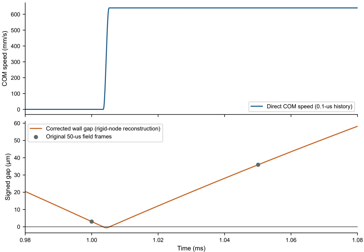
A sub-frame impact separates two non-contact field samples
