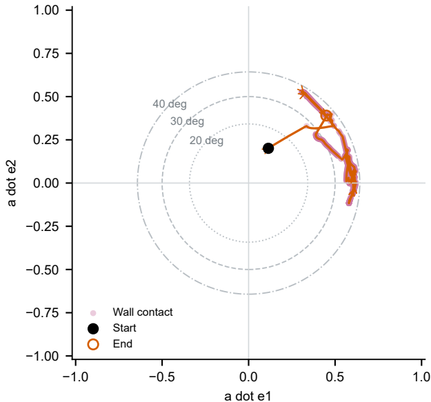
FRAME_CURRENT robot-axis local orbit
