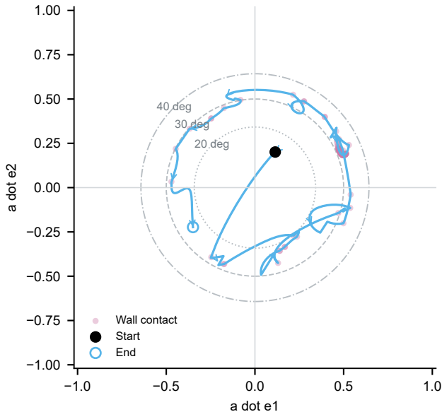
FRAME_LOCAL30_RAMP robot-axis local orbit
