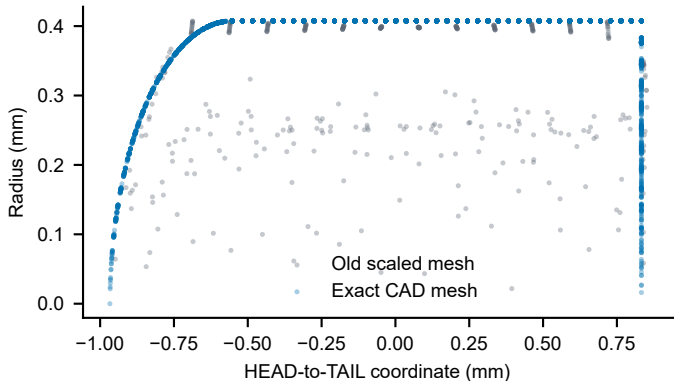
Rounded-head CAD changes volume, not nominal L/D
