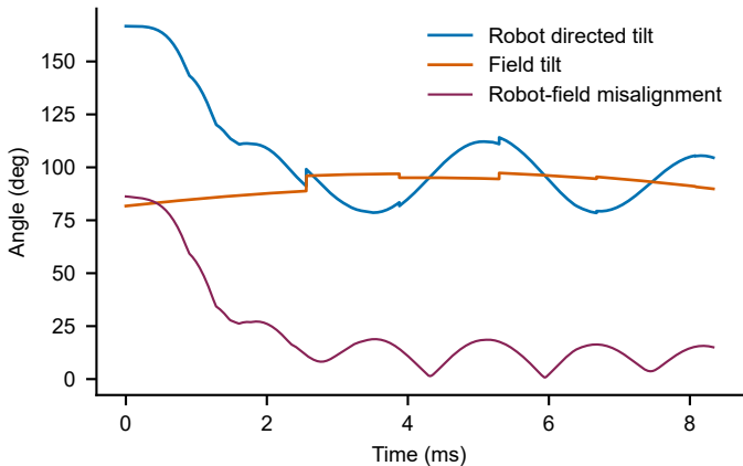
Robot overshoot is separated from field orientation
