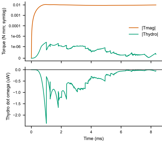
Magnetic torque persists during geometric stall
