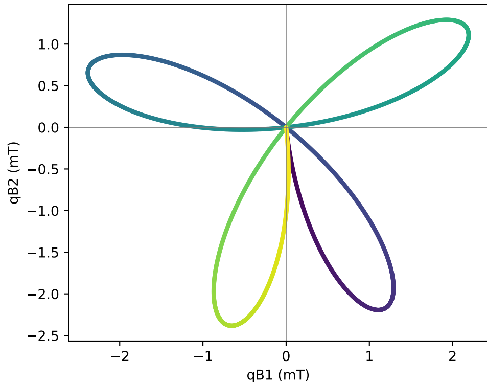
Rotating rocking field path
