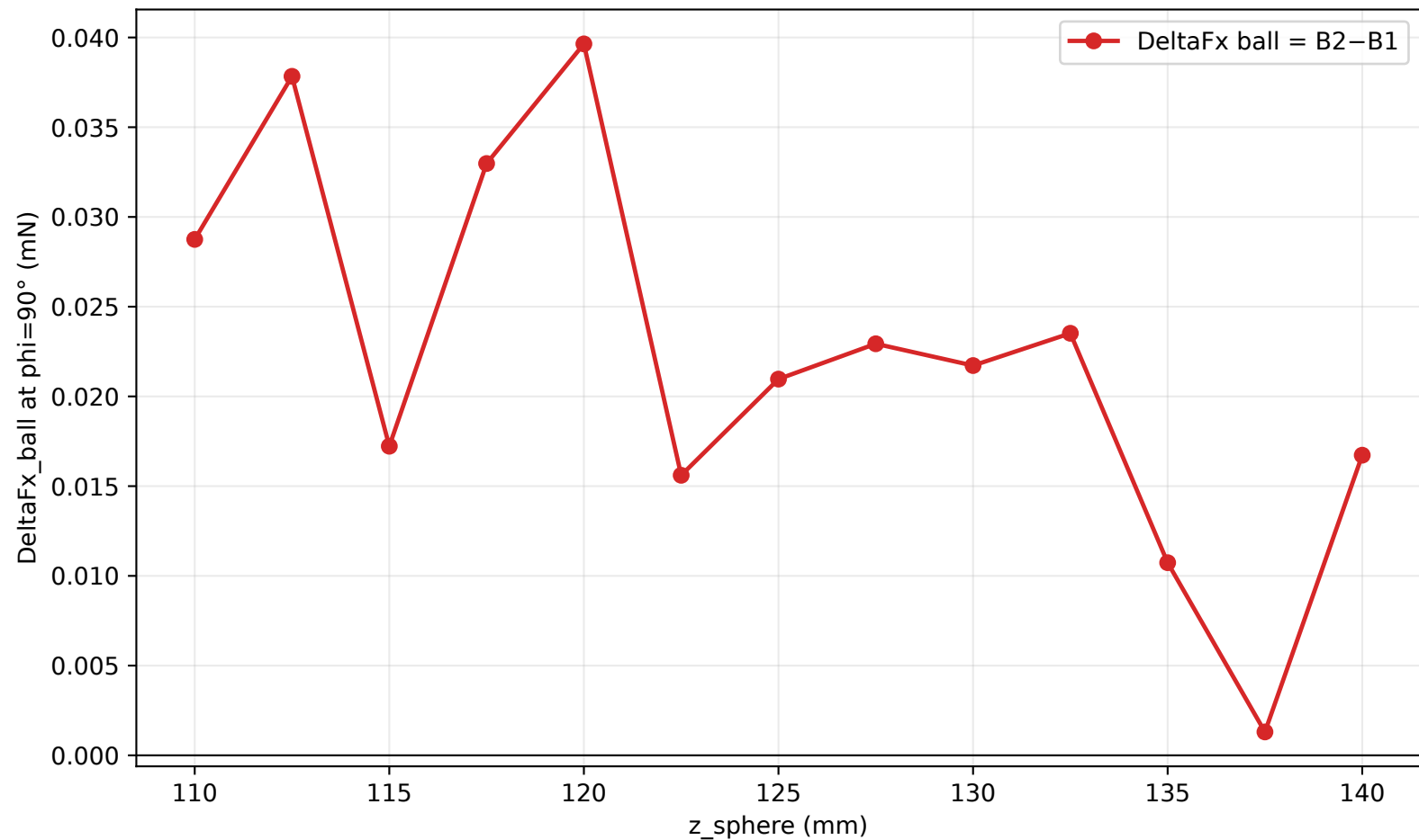
Model B: ball contribution near z=120 mm
