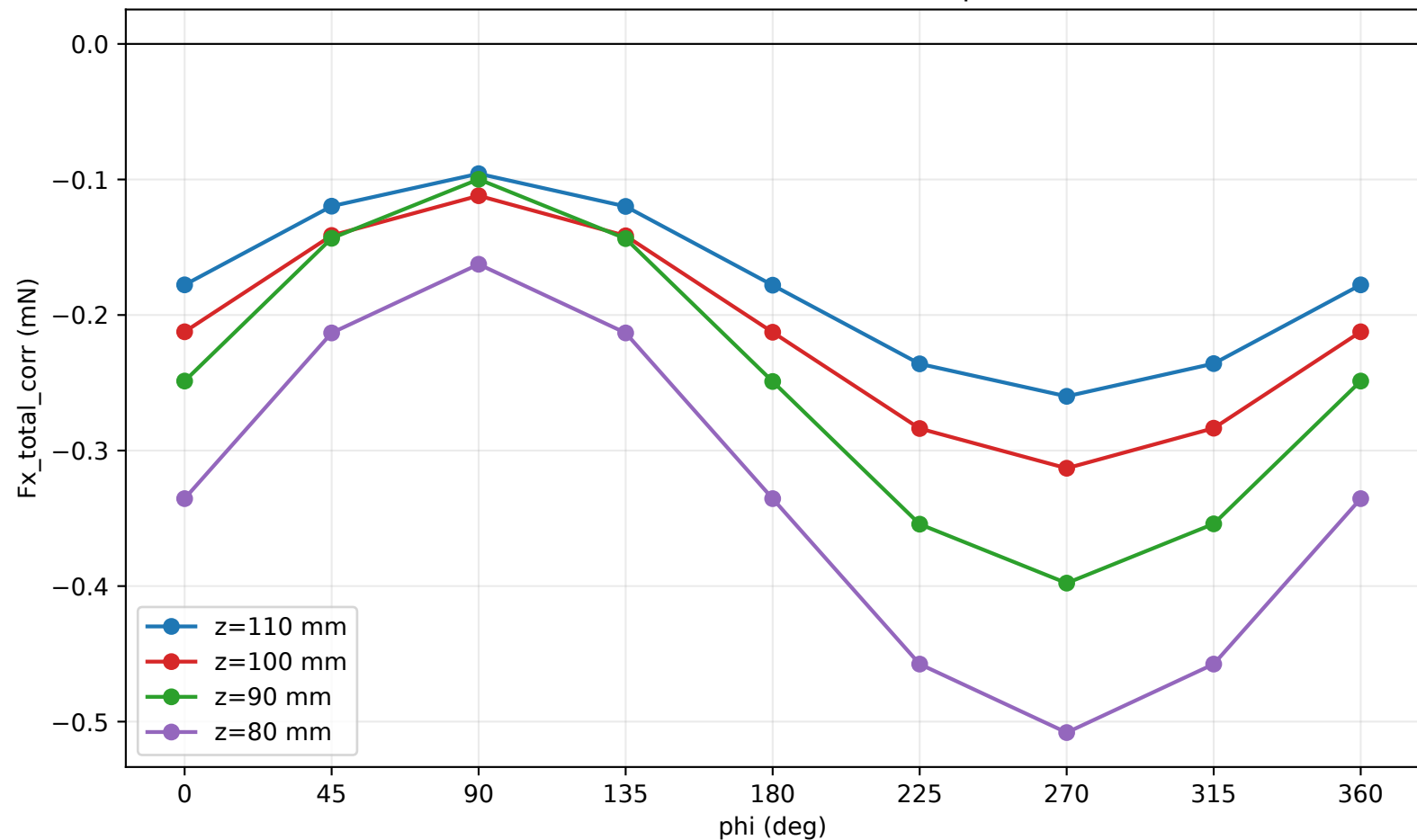
Model B: corrected force versus phase
