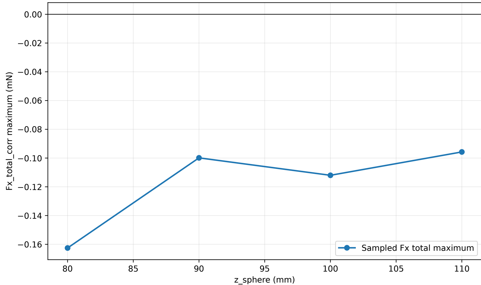
Model B: corrected cycle maximum versus height
